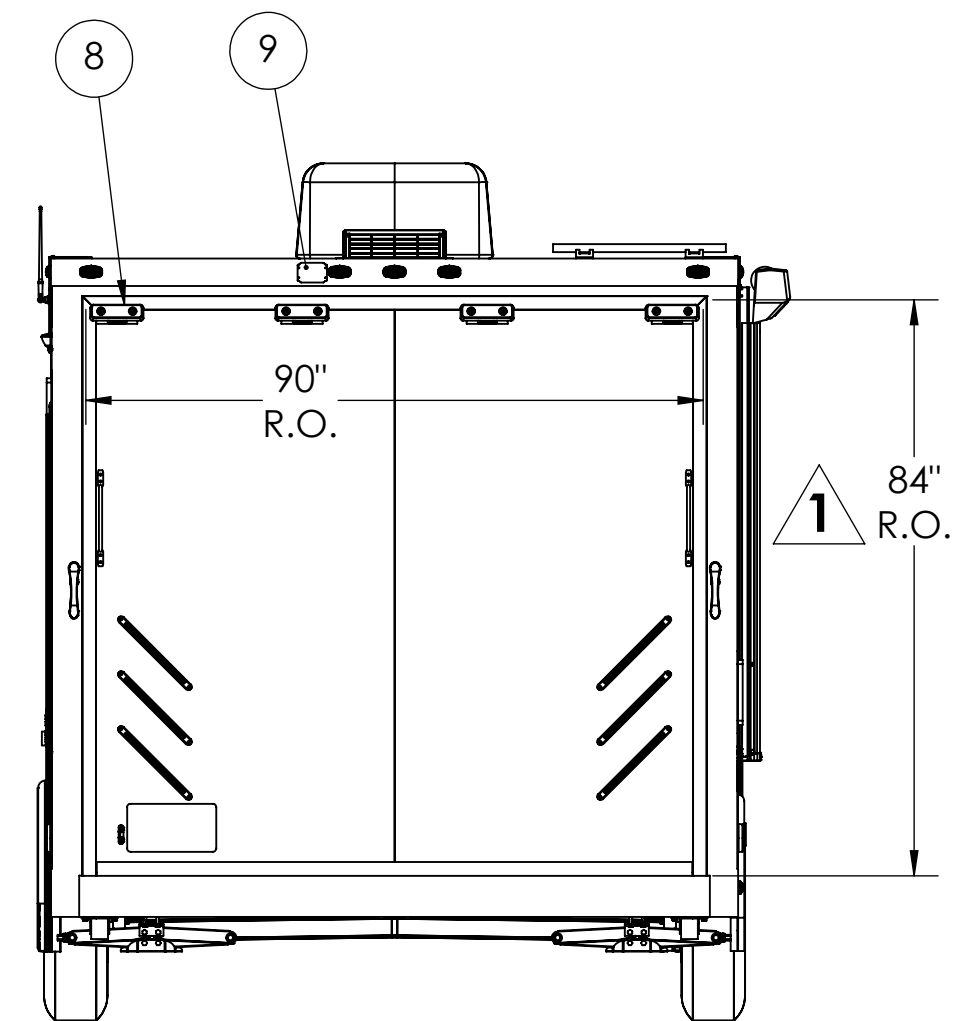
EXTERIOR REAR VIEW
