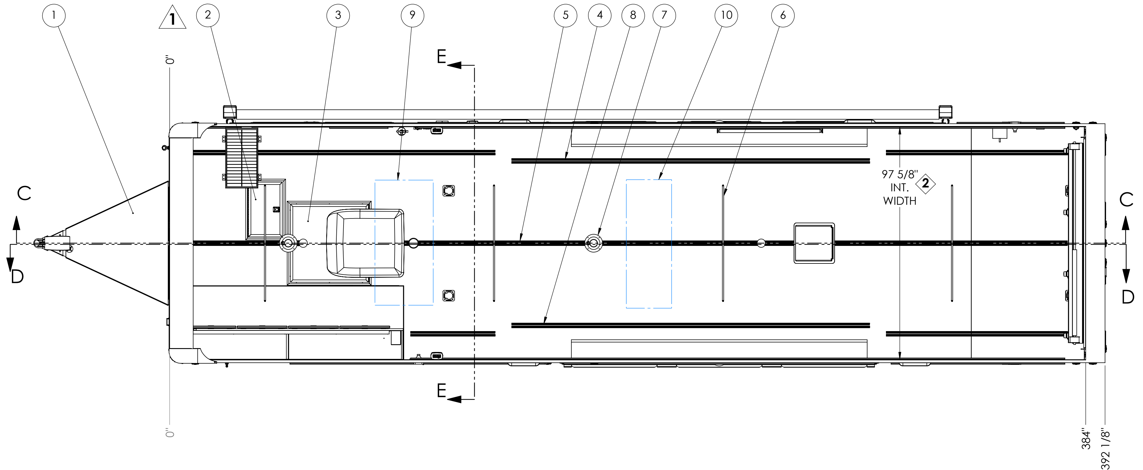
TOP VIEW POPULAR OPTIONS FLOOR LAYOUT
