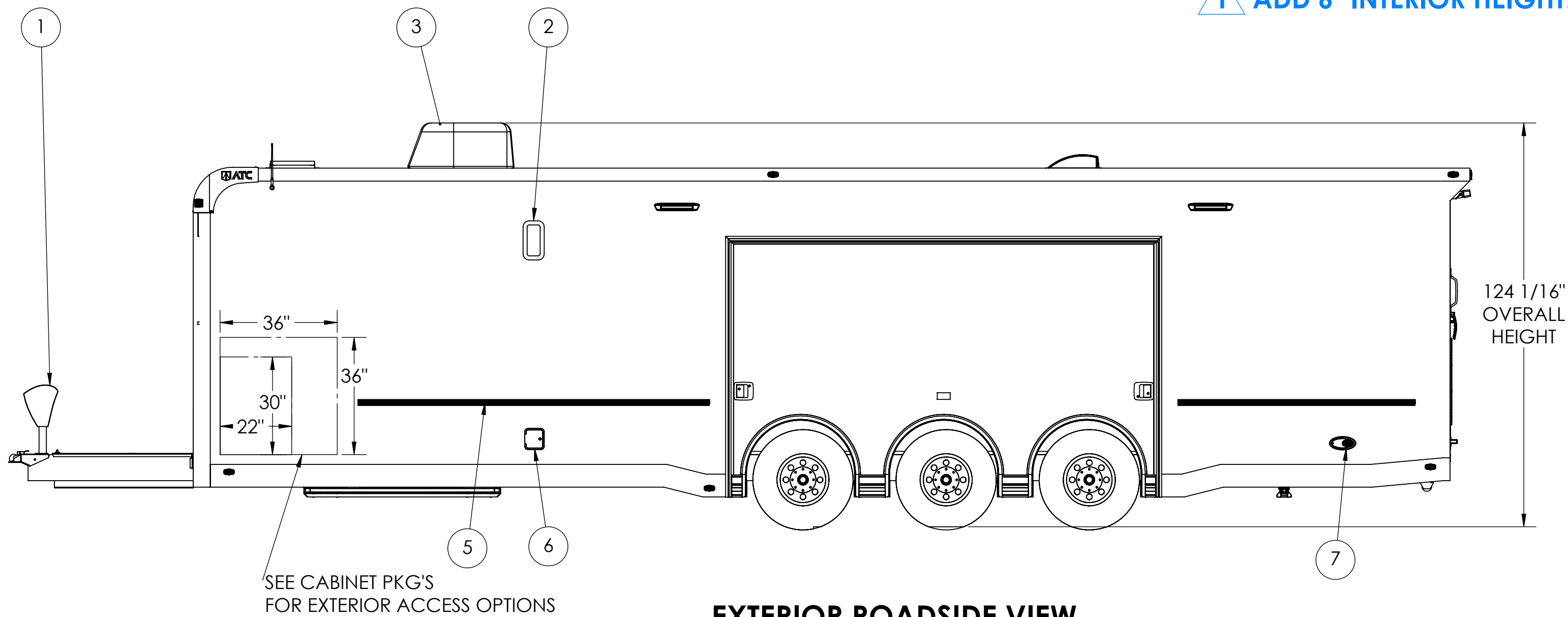
EXTERIOR ROADSIDE VIEW
