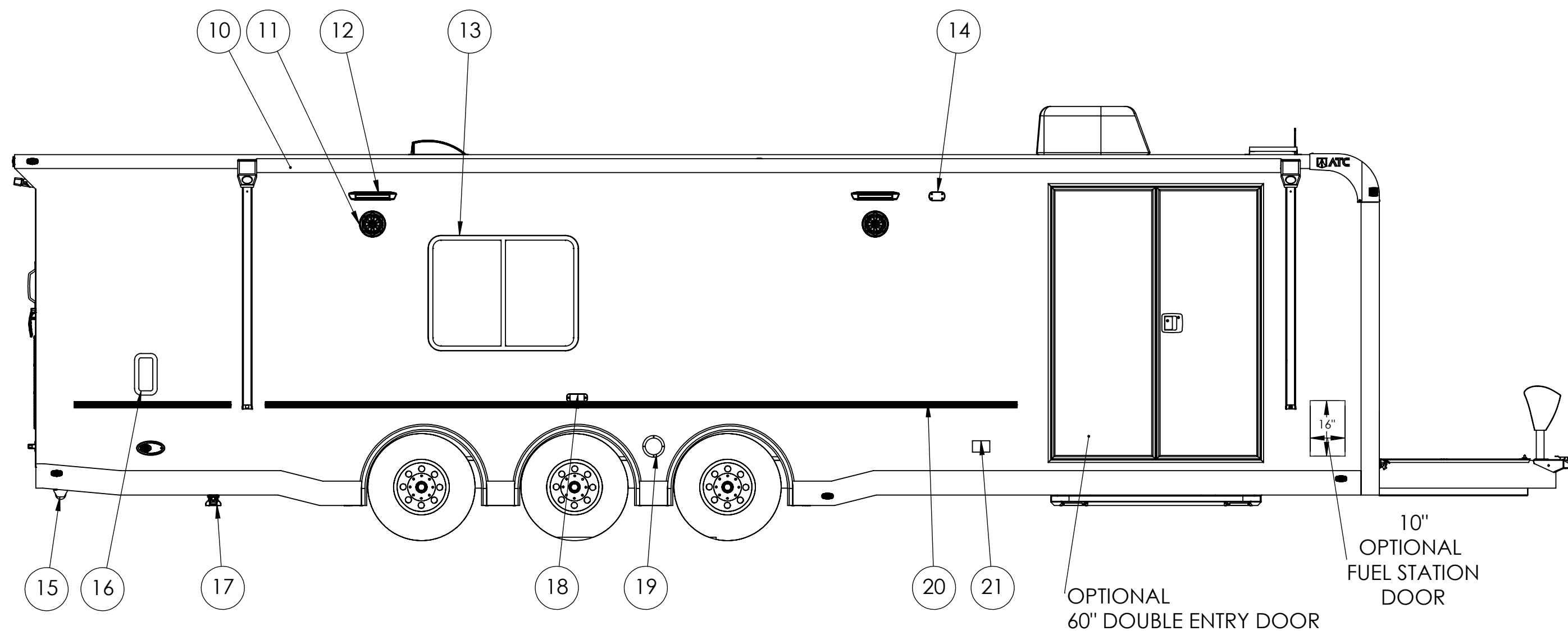
EXTERIOR CURBSIDE VIEW
